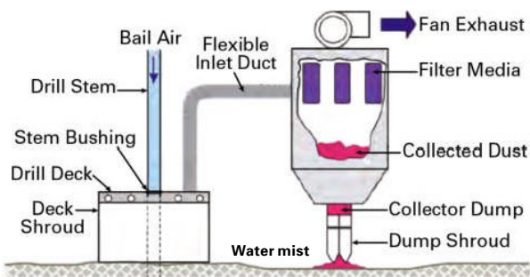
Diagram of dust control systems for rock drills, including deck shrouds for the drill bit and the discharge or dump shroud.
