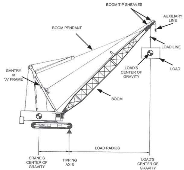
Figure 1. Key components of a typical crawler-propelled crane. The crane's weight is balanced against the weight of the lifted load. The diagram is courtesy of the Construction Safety Association of Ontario and may not be reproduced without their written permission.
